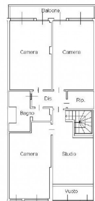
Piano 5°
